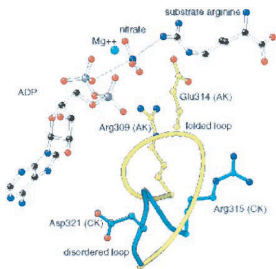
FIGURE 4 A detailed view of differences between AK loop 309–319 (yellow) and Mi6CK 315–325 (cyan) after the large domains have been superimposed. Side chains that interact with the substrates are shown by ball-and-stick models. This figure and Fig. 1 were prepared with MOLSCRIPT (Kraulis, 1991).
